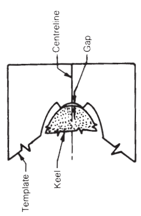
Leading edge radius of keel as shown exceeds max. tolerance.
